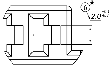
X Detay/ Detail X
