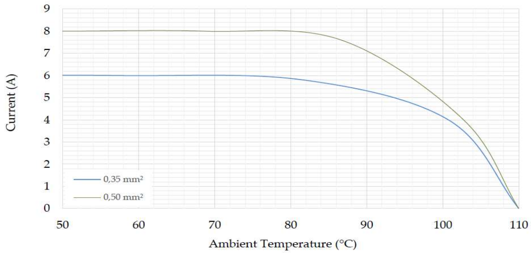
Derating Curve
